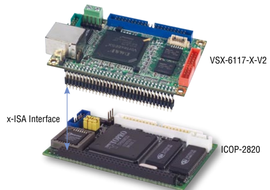
VGA function support via x-ISA interface
