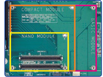
Three Sizes and Two Types (Type 6 & Type 10) Compatible
